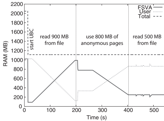
Fig. 6. Unified buffer cache. This figure shows the amount of memory consumed by the user and FSVa VMs. As applications shift their memory access pattern between file system and virtual memory usage, the unified buffer cache dynamically allocates memory among the two VMs while maintaining a constant total memory allocation.
