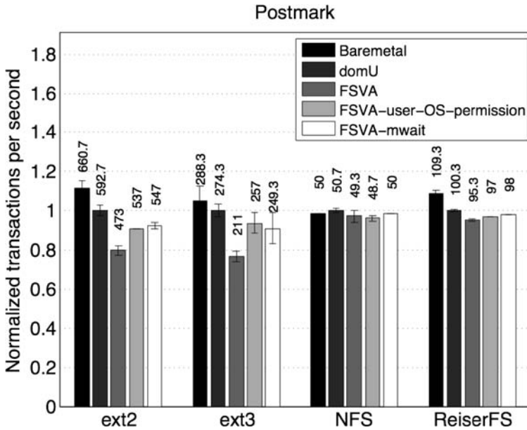
Fig. 3. Postmark results. The results are normalized on the domU results.
