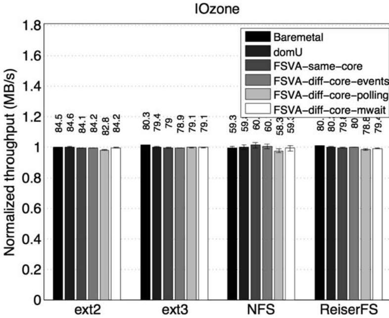
Fig. 4. IOzone results. The results are normalized on the domU results.
