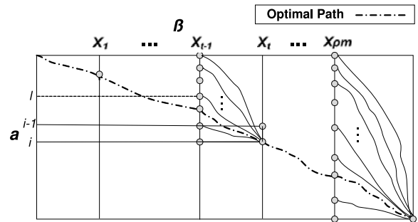
Figure 3: Proof illustration.
