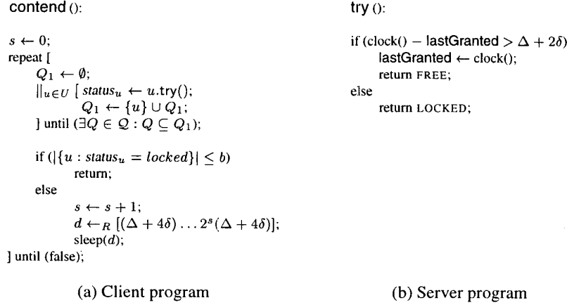
Figure 1. Mutual exclusion protocol
